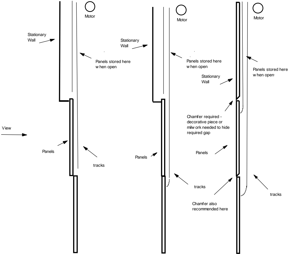
MULTI PANEL DOOR IN ONE PLANE. ONE PANEL TRAVELS STRAIGHT AND ONE PANEL TILTS DURING TRAVEL.
