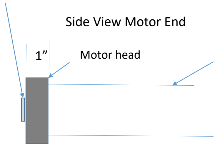
Right side steel motor brace Secures with 2 to 4 screws
